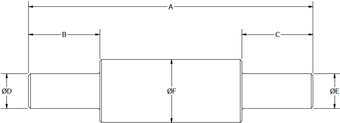
FRONT VIEW
