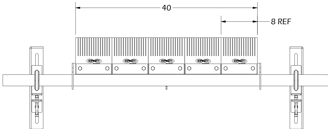
FRONT VIEW
